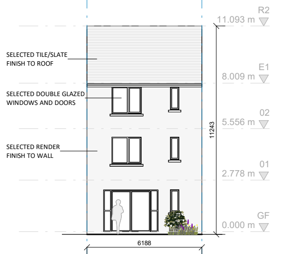
8 H08R Rear Elevation 1 : 200
