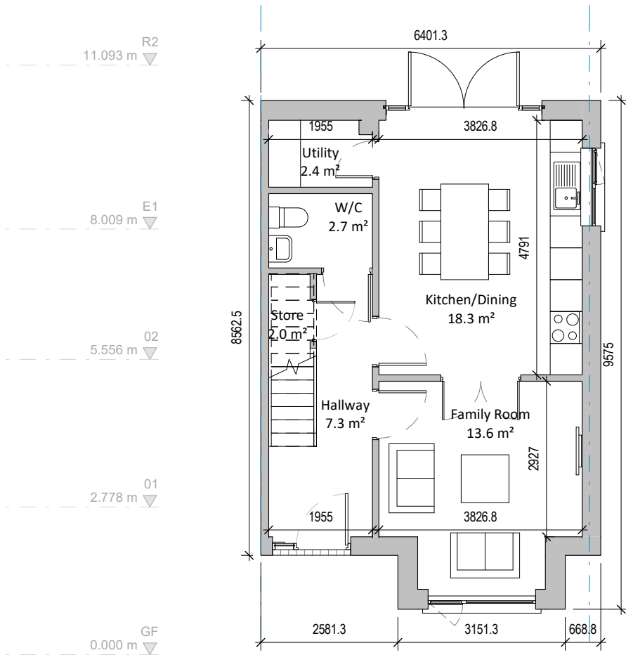
2 H08R Level 00 1 : 100
